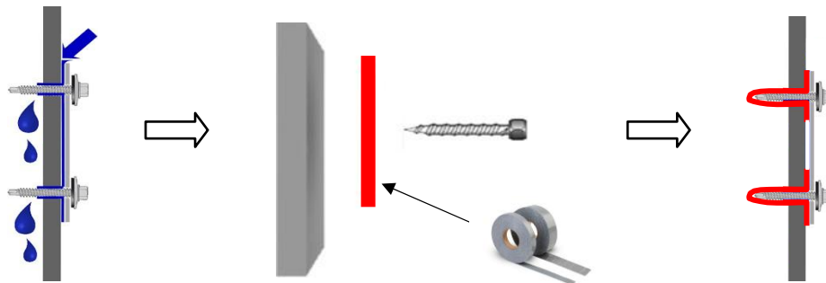
Figure 6 - Nails/screw perforations membrane sealing.
