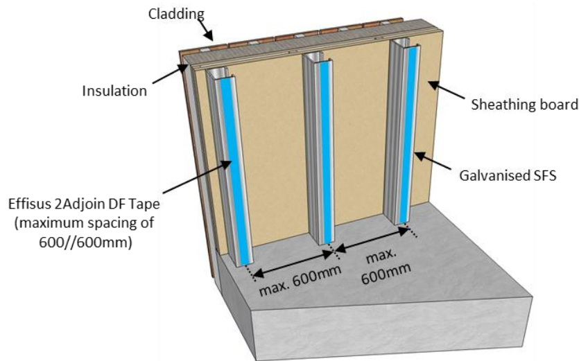
Figure 4 - Effisus Vapour FR Membrane – Fixing to the substrate
