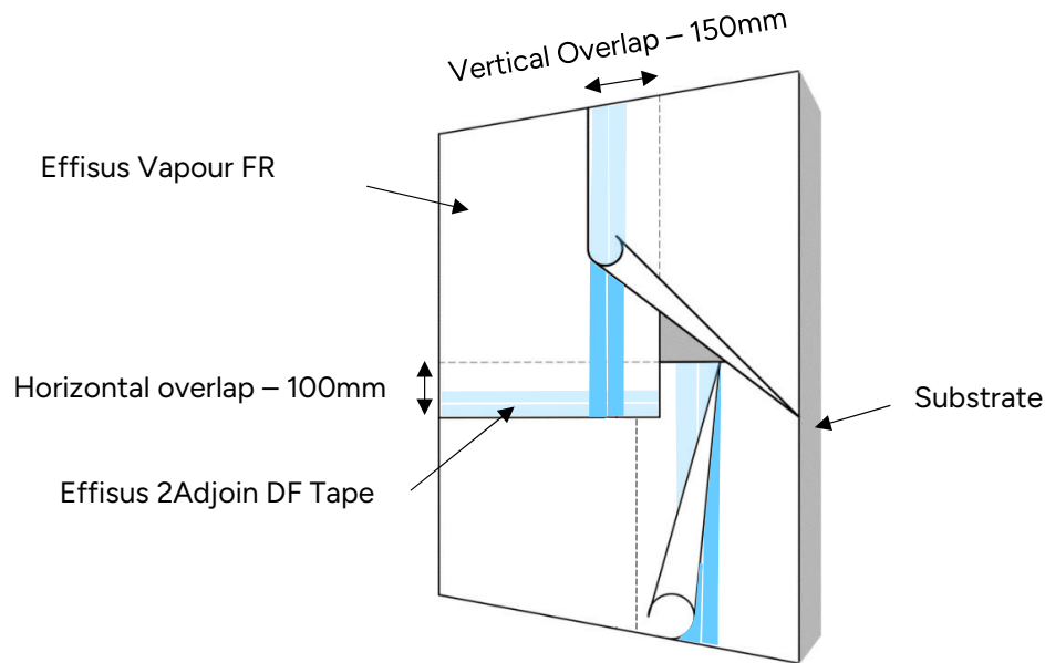
Figure 5 - Effisus Vapour FR Membrane – Overlapping Joints.
