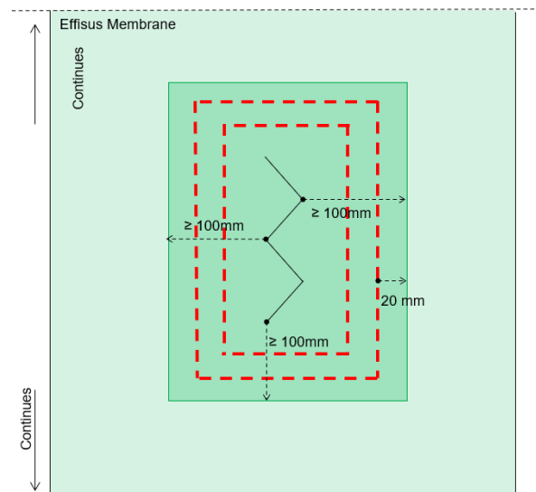
Figure 8 - Effisus Vapour FR Membrane - Repair works
