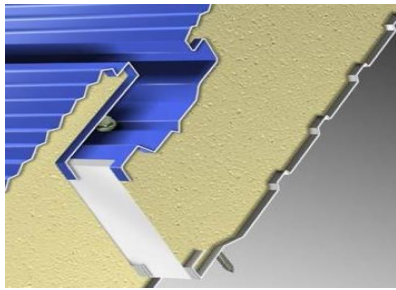
1. Sealing overlaps on sandwich panels
