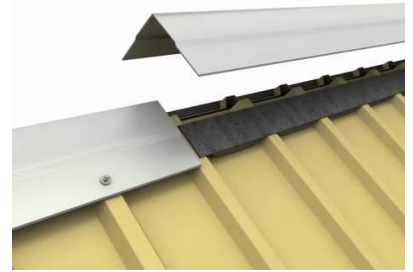
3. Sealing joints in roof ridges.
