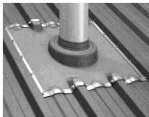
Penetrations that create barriers that stop waterflow
