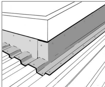
1. Sealing the roof to a parapet wall
