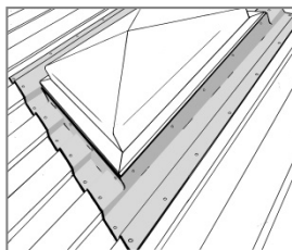
4. Sealing the roof to a skylight
