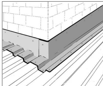
2. Sealing the roof to the facade
