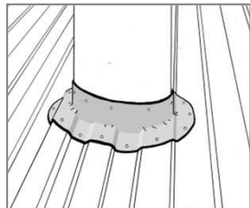
5. Sealing to a large round duct
