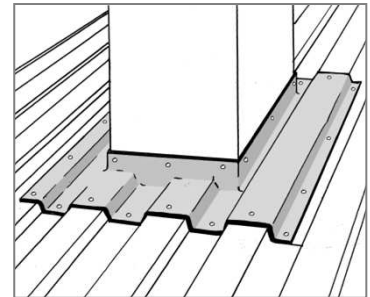
3. Sealing the roof to a square duct
