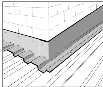
2. Sealing roofs to facades
