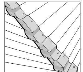
7. Sealing roof valleys
