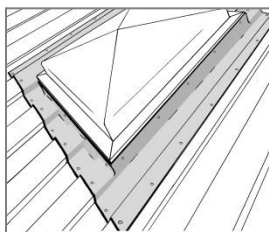
4. Sealing roofs to skylights
