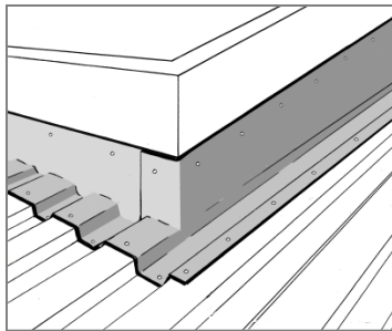
1. Sealing roofs to parapet walls
