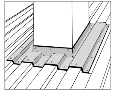
3. Sealing roofs to square ducts
